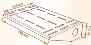
*Optional: 1*188*42*120mm Mounting Plate and Mounting Accessories
