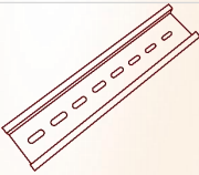
2*DIN Rail (Length: 345mm)
