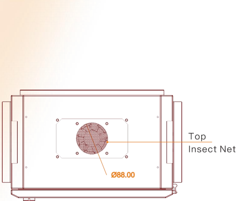
Inner Top
