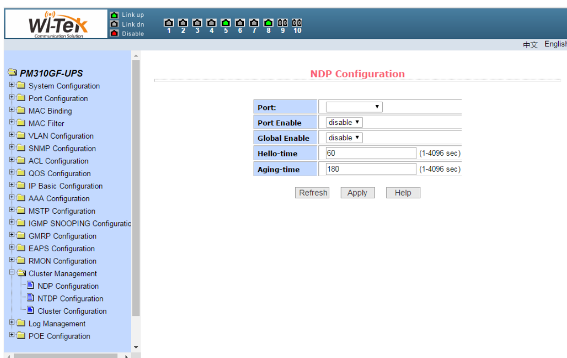
Pic 66 NDP configuration page
