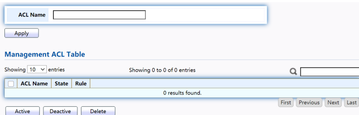
Figure 123 - Security > Management Access > Management ACL
