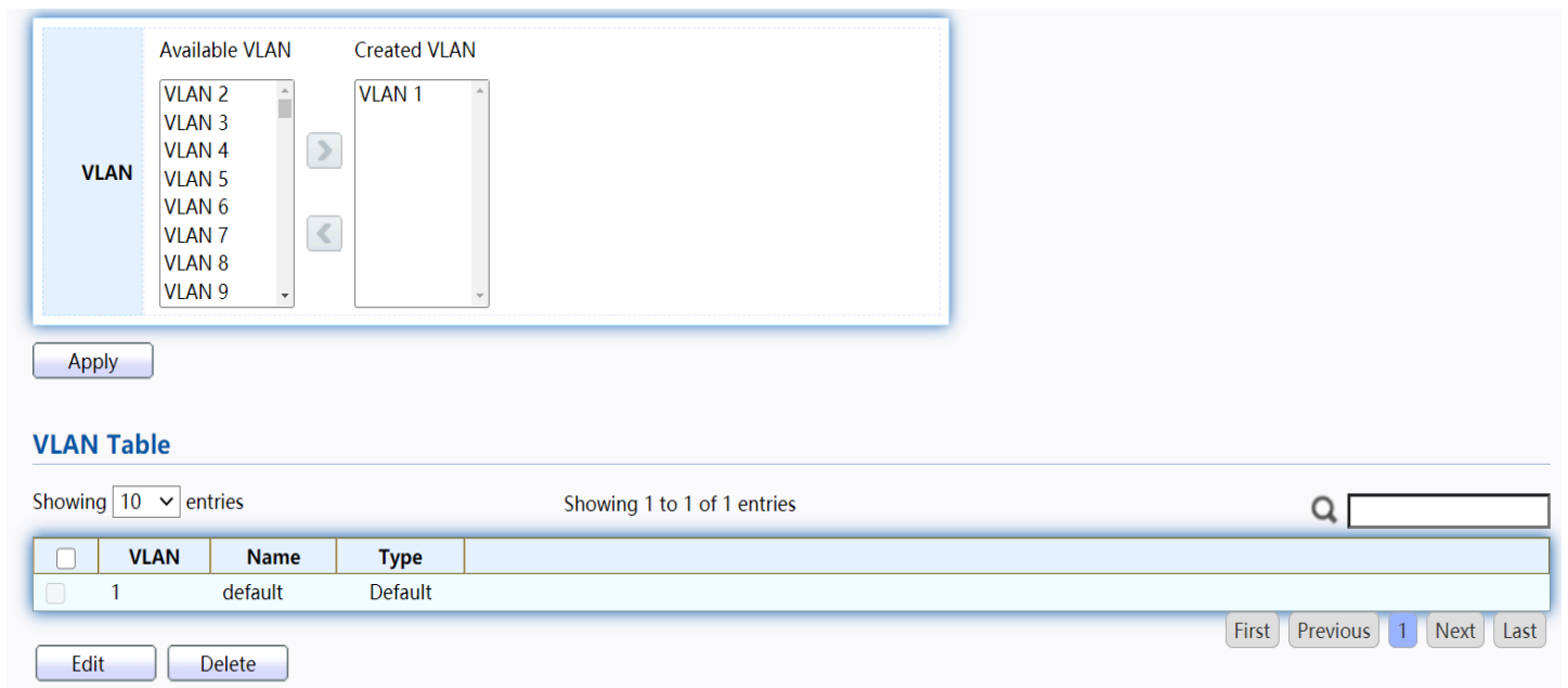
Figure 27 - VLAN > VLAN > Create VLAN
