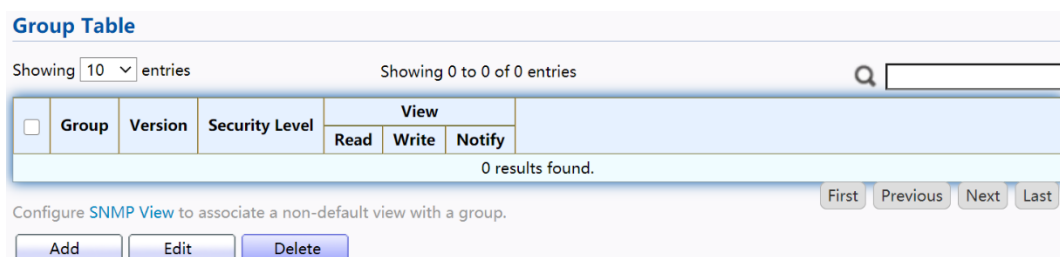
Figure 213 - Management > SNMP > Group
