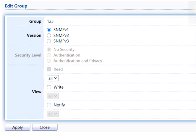
Figure 214 - Management > SNMP > Group > Add/Edit Group
