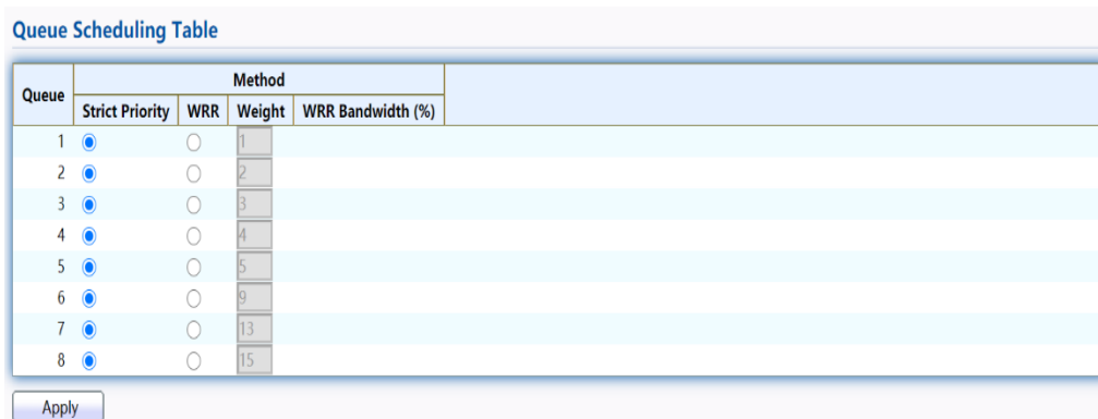
Figure 179 - QoS > General > Queue Scheduling
