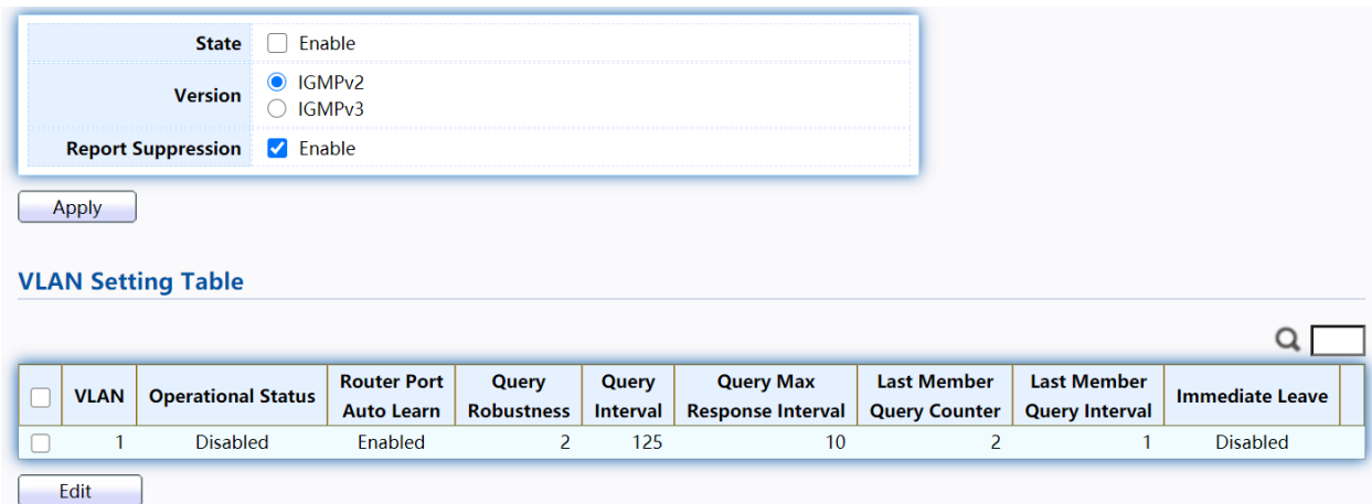
Figure 101 - Multicast > IGMP Snooping > Property
