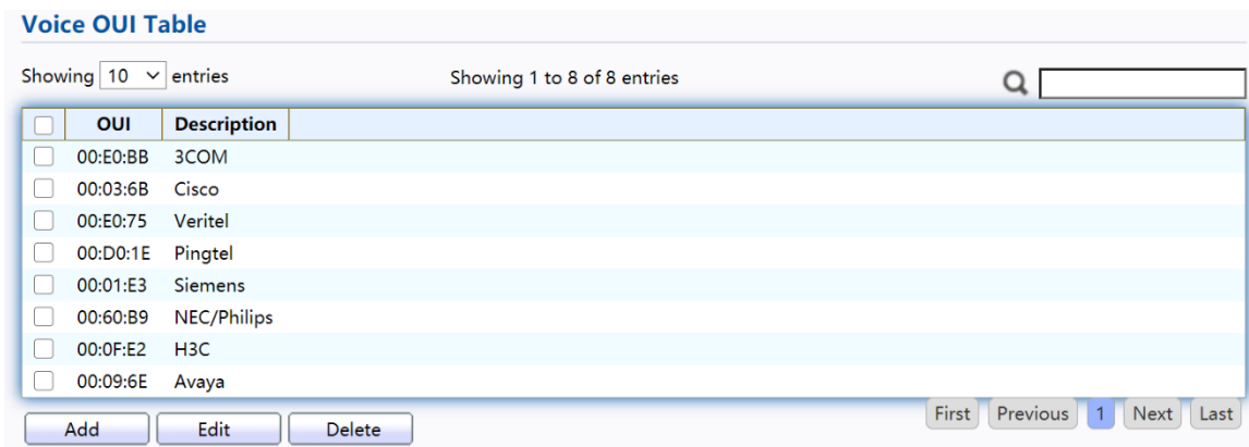
Figure 36 - VLAN > Voice VLAN > Voice OUI
