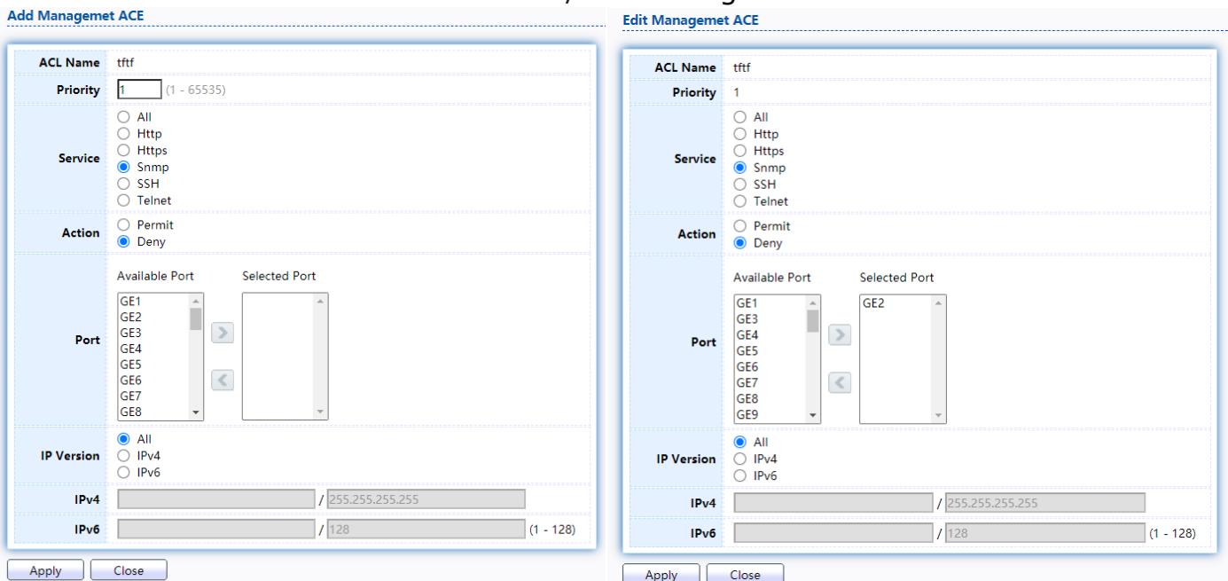
Figure 125 - Security > Management Access > Add/Edit Management ACE
